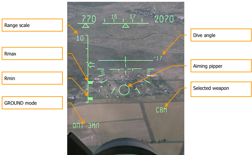
Figure 73: VISUAL GROUND mode
