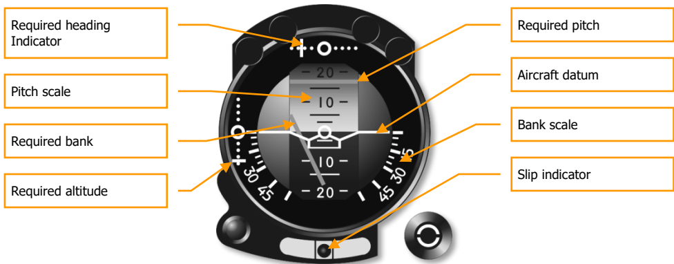
Figure 34: ADI
