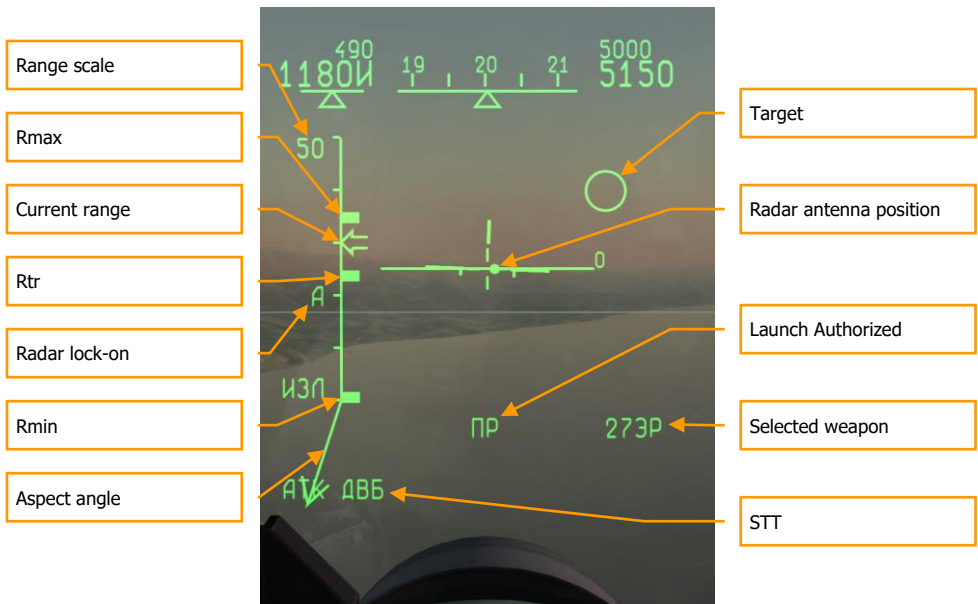
Figure 59: "АТК ДББ" (STT BVR) MODE
