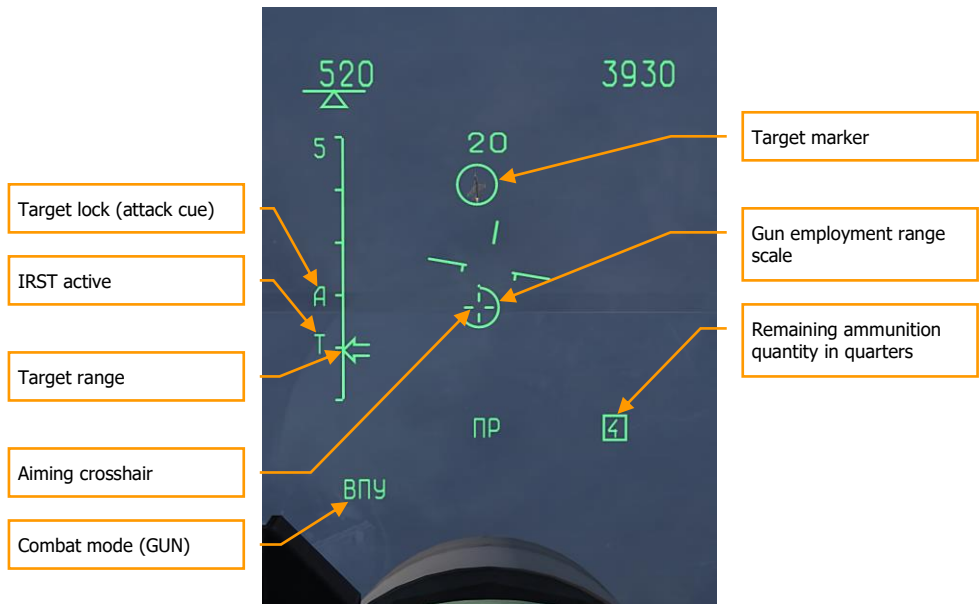
Figure 71: Lead Computed Optical Sight (LCOS) mode
