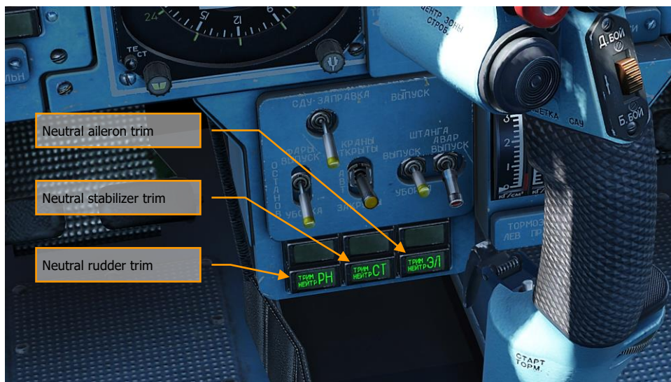
Figure 45: Trim annunciators
